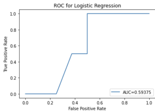
Figure 16. ROC and AUC for Logistic Regression
