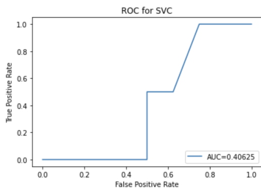
Figure 17. ROC and AUC for Support Vector Classifier
