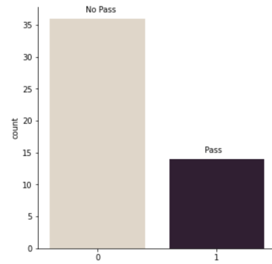
Figure 3. Pass/No Pass results distribution for 50 students
